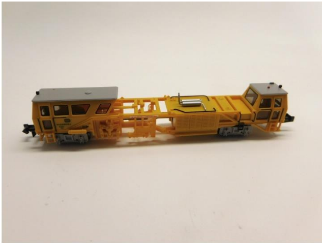
Micromotor NH022
