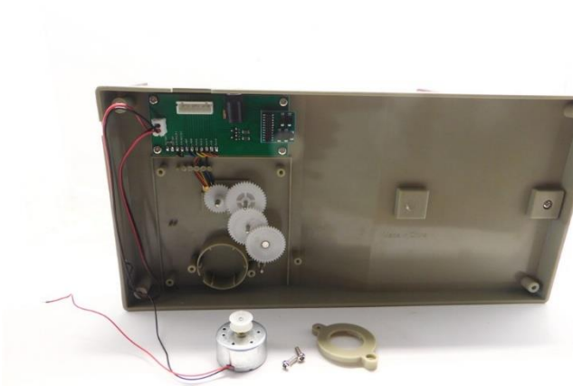
Ausbau alter Motor Take out the old motor Demonteer de oude motor
